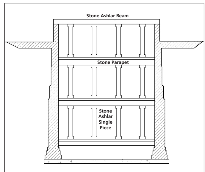
DIAGRAM 4 Sectional plan and elevation for one of the storage tank
